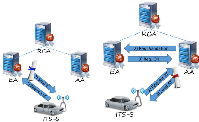
Figure 1: PKI architecture.
