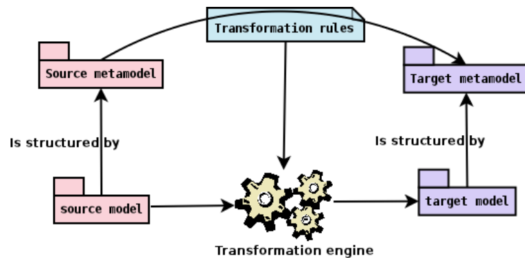
Figure 1: Simple overview of model transformation
