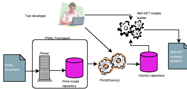
Figure 10: PNML to CAMI(x) model transformation process.
