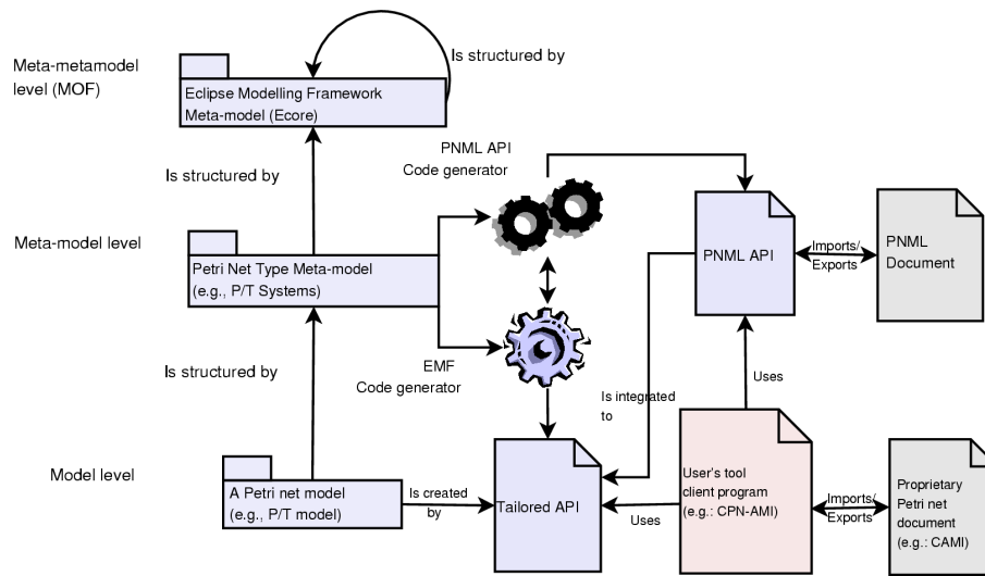
Figure 3: Overview of the production chain
