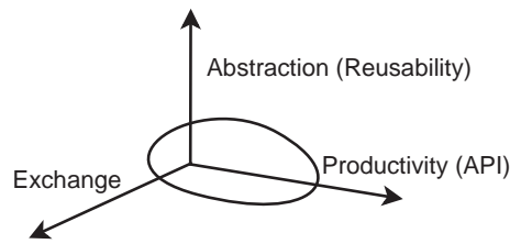
Figure 2: Metamodelling viewpoints
